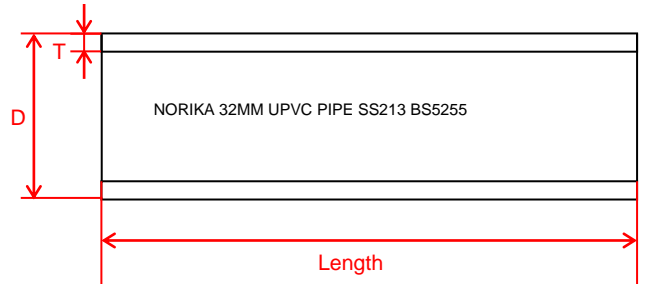
CROSS SECTIONAL VIEW
